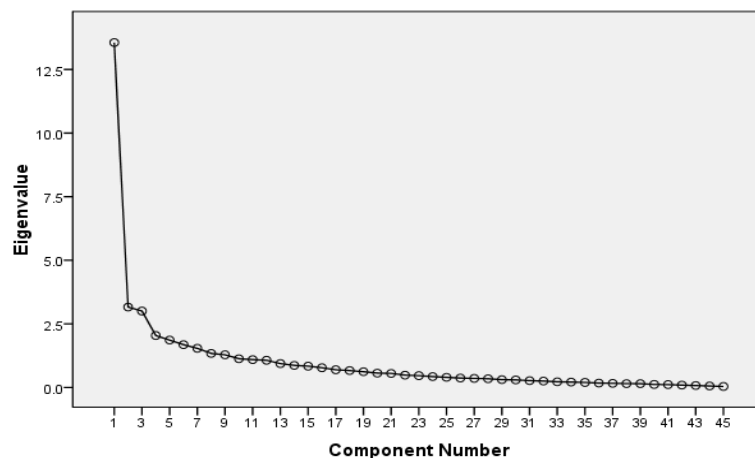
Scree Plot
